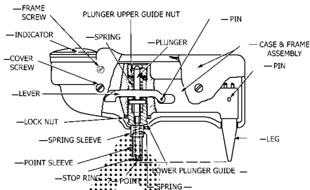
Diagram of Barcol Impressor TABLE 2 Hardness Instrument Scale Units
