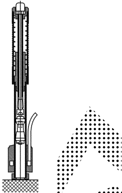
FIG. X1.1 Impact Device D
