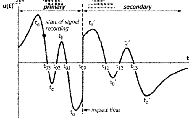
FIG. X2.1 Schematic Voltage Signal Generated By the Impact Body Travelling Through the Krautkramer Coil System
